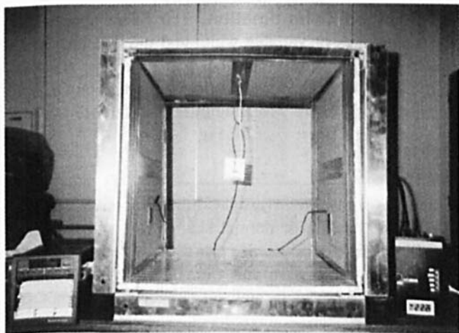
Figure 1. Photograph of the equipment of the FIR source. The FIR sources were constructed from a ceramic-coated sheet of aluminum, and the opposite side of the sheet was heated by an electric heater. FIR emitted from the ceramic-coated sheet ranged from 5.6 to 25 \mu m with a maximal intensity of 8 to 12 \mu m. The temperature in the rack was continuously monitored with a sensor placed in the rack.
