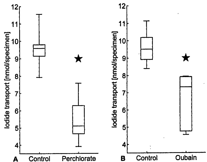
Figure 3. Boxplots showing iodide transport from the serosal to the mucosal reservoir in the presence of perchlorate 20 mM (A) or ouabain 500 \mu M (B). Initial iodide concentration was 0.2 mM. Values are nmol transported per specimen (0.64 cm 2 ) after 60 min; medians (interquartile range); whiskers drawn to the extreme values, n = 5 –7. * P < 0.01 in A and B.
