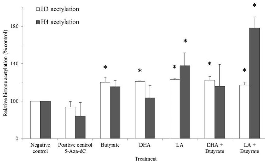
Figure 4 H3 and H4 histone acetylation (expressed as percentage of the negative control) in HCT-116 cells incubated with 5-Aza-dC (48 h), butyrate (12 h), DHA (72 h), LA (72 h), or co-treatment (see "Experiment I" section for details of Experiment I). Values are means \pm SEM. *Different from the negative control, P < 0.05 , n = 3 per treatment. The negative controls were cells incubated in media only
