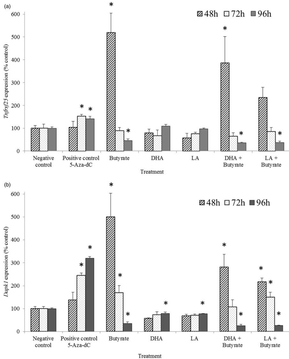
Figure 3 Time-course analysis of Tnfrsf25 (Panel a) and Dapk1 (Panel b) transcript levels (expressed as percentage of the negative control) in HCT-116 cells cultured with 5-Aza-dC, butyrate, DHA, LA, or co-treatment for 48, 72, or 96 h (see "Experiment II" section for details of Experiment II). Values are means \pm SEM. *Different from the negative control sample measured at the same time point, P < 0.05 , n = 3 per treatment. The negative controls were cells incubated in media only
