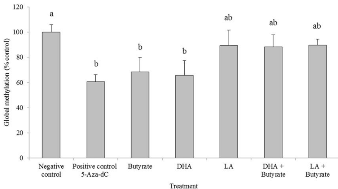
Figure 2 Global DNA methylation status (percent of the negative control) in HCT-116 cells cultured with 5-Aza-dC (48 h), butyrate (12 h), DHA (72 h), LA (72 h), or co-treatment (see “Experiment I” section for details of Experiment I). Values are means \pm SEM. Values not sharing common letters are significantly different, P < 0.05, n = 6 per treatment. Negative controls represent cells incubated in media only. DHA: docosahexaenoic acid; LA: linoleic acid
