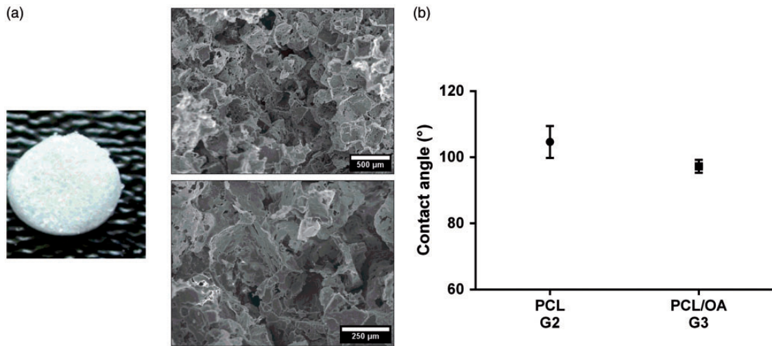
Figure 1 PCL and PCL/OA scaffolds (a) Macroscopic sample picture, on details surface porosity of PCL/OA composition scale bar 500 and 250 µm; (b) Contact angle values 104.6 \pm 3.5^\circ and 97.3 \pm 1.3^\circ PCL and PCL/OA, respectively
