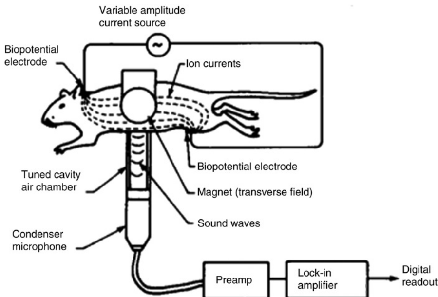
Figure 2 An experiment for the magneto-acoustic detection of current in a hamster. From Towe and Islam. 6 (© 1988 IEEE)
