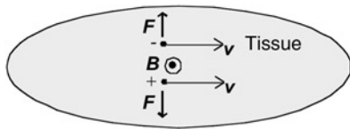
Figure 3 A motion-induced voltage. Tissue is moving with speed v to the right in the presence of a magnetic field B directed out of the paper. Negative ions experience an upward Lorentz force, and positive ions experience a downward Lorentz force. The resulting charge separation produces a negative voltage at the top of the tissue and a positive voltage at the bottom
