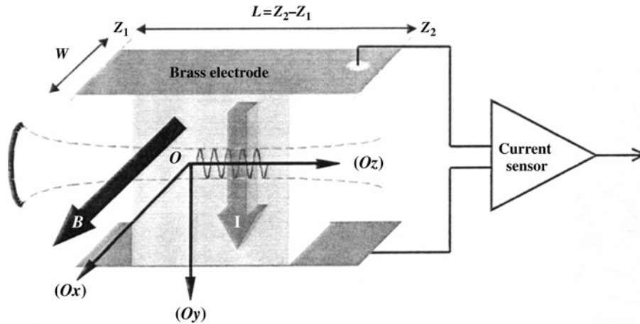
Figure 5 Schematic diagram of the experimental setup for detection of currents caused by the ultrasonically-induced Lorentz force. Axis Oz is the ultrasound propagation axis, Ox has the same orientation as the magnetic field, and the interaction current is positive along Oy . The origin, O , is located at the focal point of the transducer. From Montalibet et al. 16
