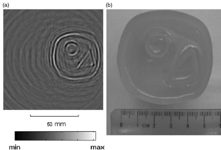
Figure 7 (a) The two-dimensional MAT-MI image of a gel phantom, with two columns of 0% salinity gel embedded in gel of 10% salinity. (b) Top view photo of the phantom. From Li et al. 25 (© 2007 IEEE)
