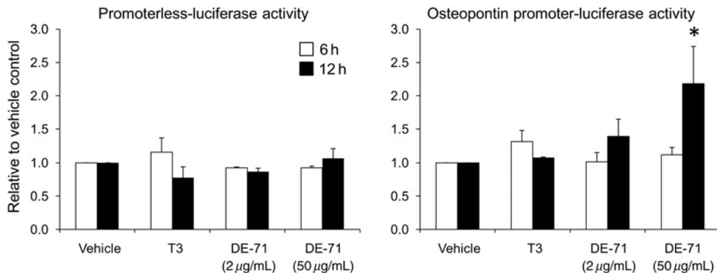
Figure 4 Effects of T3 (10 nmol/L) and DE-71 (2 and 50 \mu\text{g/mL} ) on relative activity of the promoterless luciferase (paLuc) and osteopontin gene promoter-luciferase (OPN-Luc) constructs plotted as fold change with respect to vehicle control (activity = 1.0). Bars represent mean plus SEM. * P < 0.05 compared with vehicle control for OPN-Luc. For paLuc n = 2 experiments. For OPN-Luc n = 5 separate experiments except n = 4 for DE-71 (2 \mu\text{g/mL} )
