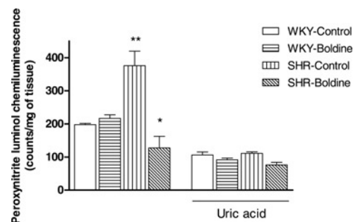
Figure 3 Levels of peroxynitrite generation in aortic rings from control and boldine-treated Wistar-Kyoto rats (WKY) and spontaneously hypertensive rats (SHR). Results are mean \pm SEM ( n = 4-6 ). ** P < 0.01 compared with WKY-Control. * P < 0.01 compared with SHR-Control
