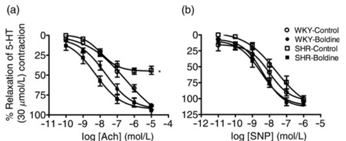
Figure 1 Endothelium-dependent and -independent relaxations to acetylcholine (ACh, a) and sodium nitroprusside (SNP, b), respectively, in aortic rings isolated from control and boldine-treated Wistar-Kyoto rats (WKY) and spontaneously hypertensive rats (SHR). Data are expressed as mean \pm SEM ( n = 6–7). 5-HT, 5-hydroxytryptamine. * P < 0.001 compared with respective control group
