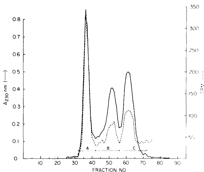
FIG. 1. Elution profile of collagen Types I and III separated on an A-5 M column ( 1 \times 150 cm). Approximately 15 mg of purified collagen was applied to the column and the percentage Type III (Region A) was determined by dividing the radioactivity in Region A by the total radioactivity in Regions A, B, and C.
