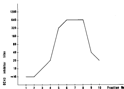
FIG. 4. Distribution of the OC43 inhibitor in fractions collected after sucrose density gradient centrifugation of a lot of fetal calf serum.
