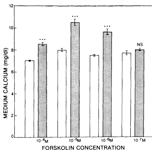
FIG. 1. Effect of forskolin on calcium release from neonatal mouse half calvaria in vitro . Half calvaria were cultured for 96 hr in media containing 1 \times 10^{-4} , 1 \times 10^{-5} , 1 \times 10^{-6} , 1 \times 10^{-7} M forskolin or vehicle alone. Media were changed at 48 hr. Values shown represent the mean media calcium concentrations for 5 half calvaria per group at 96 hr incubation. Vertical bars are SE. NS: not significantly different from control group ( P > 0.05 ); ***significant at P < 0.001 , when compared to control group. (□) Control group; (▒) forskolin group.
