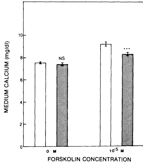
FIG. 4. Effect of acetazolamide on forskolin-induced calcium release. Half calvaria were cultured for 96 hr in media containing vehicle or 1 \times 10^{-5} M ( \square ) forskolin or forskolin at this concentration in the presence of 1 \times 10^{-4} M ( \square ) acetazolamide. The media were changed at 48 hr. The values shown are mean media calcium concentrations of 5 half calvaria per group at 96 hr incubation. The vertical bars are SE. NS: not significantly different from control group (no forskolin, no acetazolamide; P > 0.05 ); ***significant at P < 0.001 , when compared to acetazolamide control (no forskolin) group. Forskolin significantly ( P < 0.01 ) increased the medium calcium in the acetazolamide-treated cultures indicating that inhibition was incomplete.
