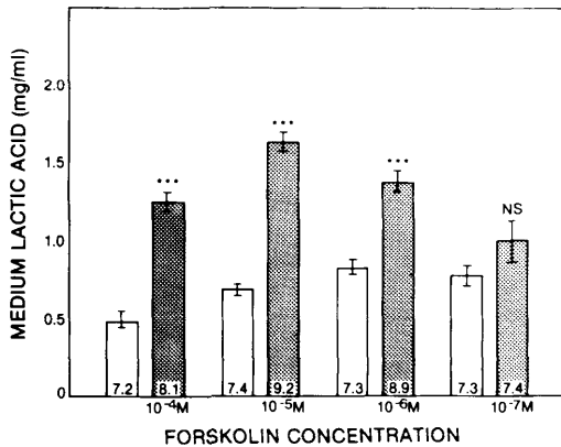
FIG. 2. Lactate release by cultured neonatal mouse half calvaria in response to forskolin. Half calvaria were cultured for 96 hr in media containing 1 \times 10^{-4} , 1 \times 10^{-5} , 1 \times 10^{-6} , and 1 \times 10^{-7} M forskolin or vehicle alone. Media were changed at 48 hr. Lactic acid and calcium concentrations were determined in the media after 96 hr of incubation. Values shown are mean media lactic acid concentrations for 5 half calvaria per group at 96 hr. Vertical bars are SE. The values inside the bars represent the mean media calcium concentrations during the same period of incubation. NS: not significantly different from control group ( P > 0.05 ); ***significant at P < 0.001 , when compared to control group. (□) Control group; (▨) forskolin group.
