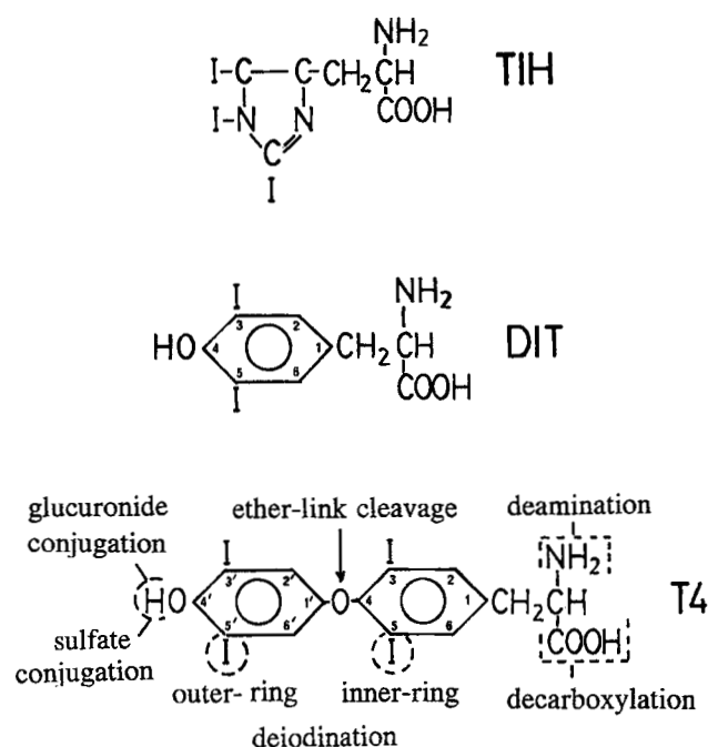
Figure 1. Structures of selected iodoamino acids. TIH, 1,2,5-triiodo-histidine; DIT, 3,5-diiodotyrosine; T 4 , L-thyroxine. Various degradative pathways are shown for T 4 . Two other commonly encountered iodoamino acids not shown above are MIT (monoiodotyrosine, which lacks the 5-iodine of DIT) and T 3 (3,5,3'-triiodo-L-thyronine, which is formed from T 4 by removing the 5' iodine).
