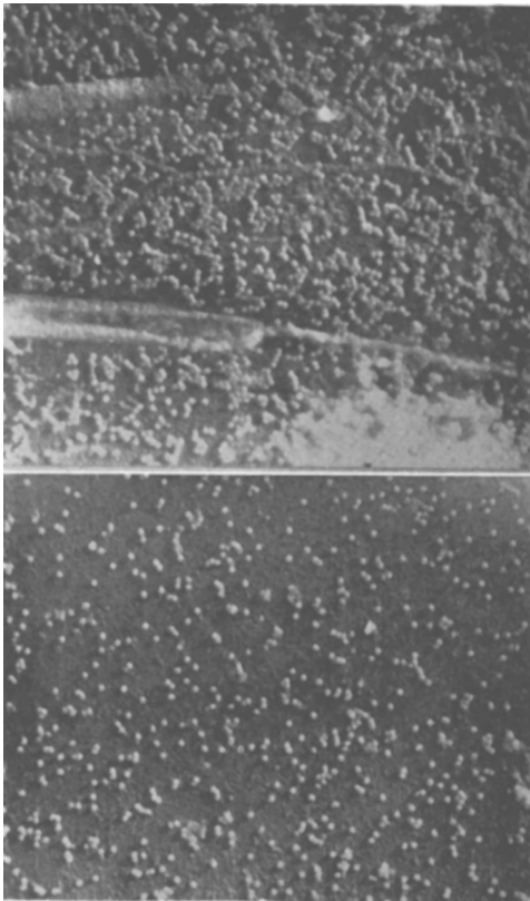
FIG. 2. (top). Chromium shadowed preparation of the same slide. Individual particles may be seen breaking off cell at bottom. \times 10,300 .
