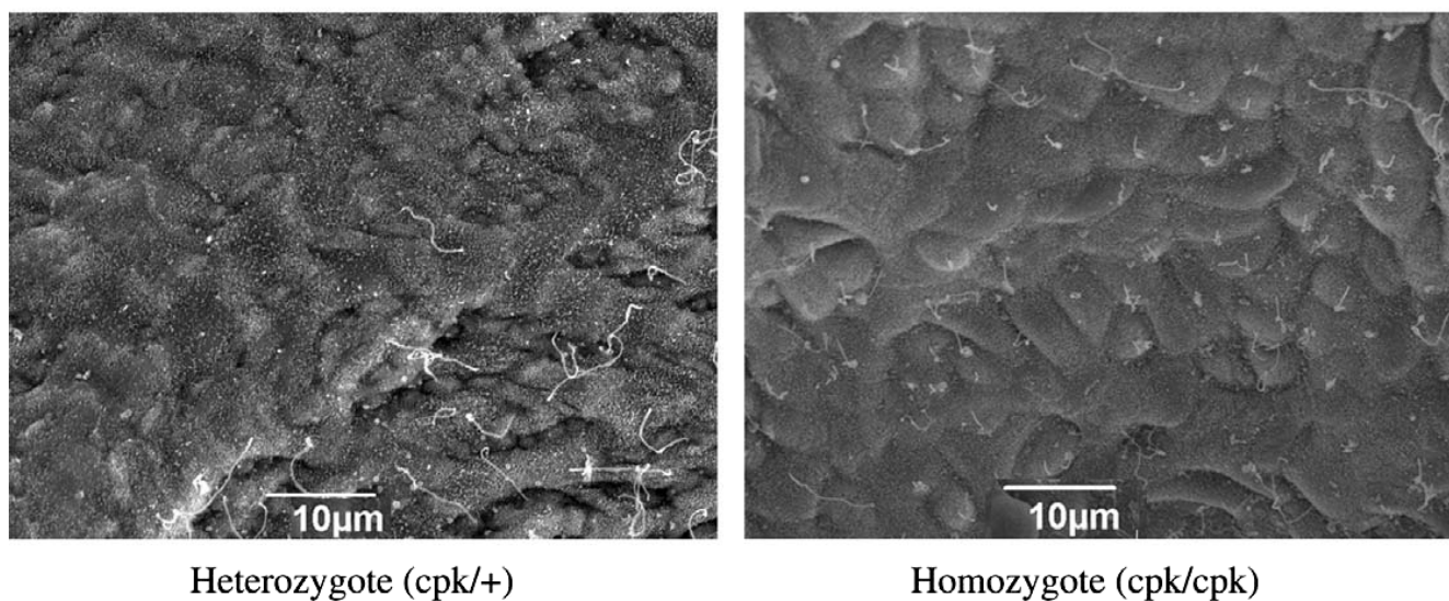
Figure 4. SEM of bile ducts/cysts from BALB/c-cpk mice. The micrographs of bile ducts from normal, heterozygous-cpk/+ and homozygous-cpk/cpk mice (top micrographs) all possess ciliated epithelia; however, the cilia in the normal mice all appear roughly the same length while cilia in heterozygous and homozygous mice are quite variable in length. In the cysts from heterozygous and homozygous mice (bottom micrographs), the variability in cilia length is very obvious, from being almost non evident to cilia that are very long.
